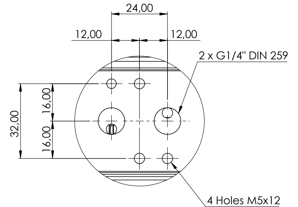
DETAIL B SCALE 1 : 1
